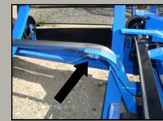
FILM SENSOR SHUTDOWN STOPS WRAPPER WHEN OUT OF FILM
