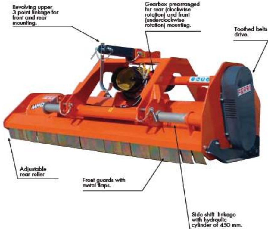
Revolving upper 3 point linkage for front and rear mounting.
