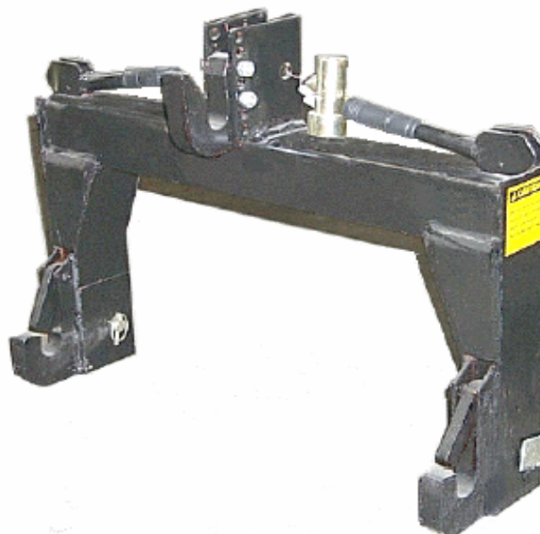
QH-101 Cat. 1 Quick Hitch
