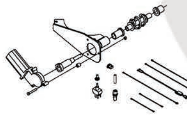
ELECTRIC ROTATION
