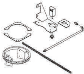
HYDRAULIC ROTATION
