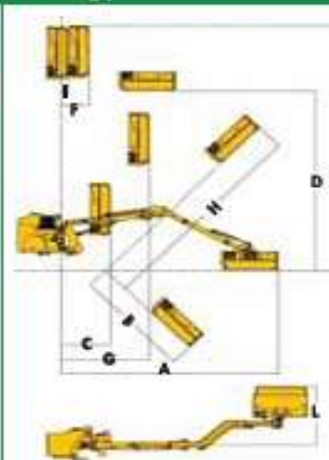
TNS 125 direct drive
